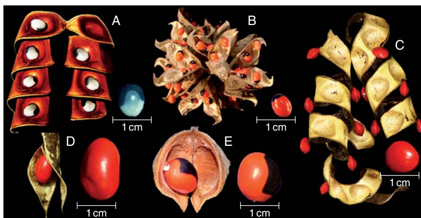
FIG. 1. Pods and mimetic seeds of Abarema langsdorffii (A), Abrus precatorius (B), Adenanthera pavonina (C), Erythrina velutina (D) and Ormosia arborea (E).
