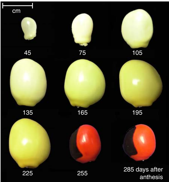
FIG. 4. Ormosia arborea seeds from different harvesting times during seed development.
